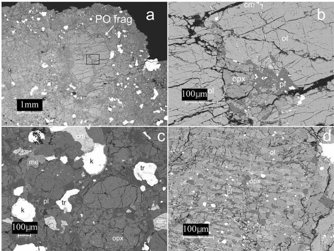
Fig. 7. Backscattered electron images of the Villalbeto de la Peña meteorite: a) Portion showing a recrystallized porphyritic olivine chondrule fragment. White grains are metallic Fe-Ni, troilite and chromite. b) Area outlined in Fig. 7a showing a plagioclase-rich melt (pl), numerous impact-induced fractures (black) and coarse grains of olivine (ol) and orthopyroxene (opx). c) Typical recrystallized region showing: kamacite (k), troilite (tr), chromite (cm) and merrillite (me). d) Recrystallized barred olivine chondrule with discontinuous olivine bars, intercalated orthopyroxene, and blebs of metallic Fe-Ni (white).
